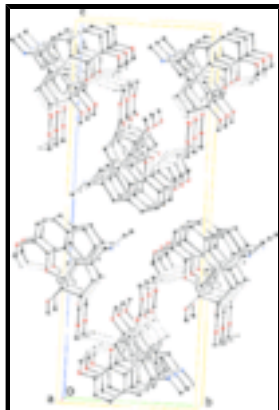
Fig. 4. A partial packing diagram of the title compound. Hydrogen bonds are shown as dashed lines. H atoms not involved in hydrogen bonding have been omitted.
