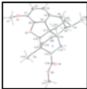
Fig. 1. The molecular structure of the title molecule, with the atom-numbering scheme. Displacement ellipsoids are drawn at the 20% probability level.
