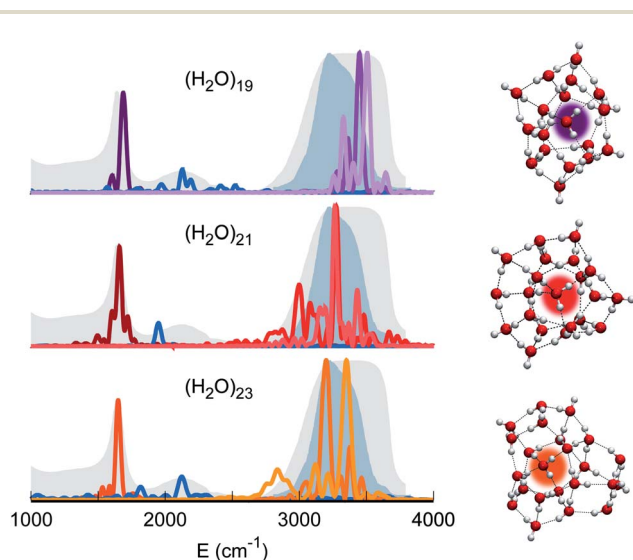
Fig. 4 Power spectra of the target monomer for larger clusters. The peaks corresponding to bendings, stretches, and combined bending-libration bands of (\text{H}_2\text{O})_{19} (top), (\text{H}_2\text{O})_{21} (middle), and (\text{H}_2\text{O})_{23} (bottom) are reported.
