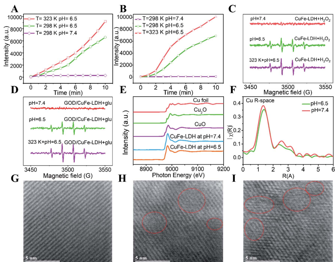
Fig. 3 The reaction of TA with the generated \cdot\text{OH} -induced enhancement of fluorescence (A) CuFe-LDHs and \text{H}_2\text{O}_2 at pH = 7.4, 6.5, 6.5 + 323 K; (B) GOD/CuFe-LDHs and glucose at pH = 7.4, 6.5, 6.5 + 323 K. (C) ESR spectra of CuFe-LDHs by adding \text{H}_2\text{O}_2 in buffers at various pH values. (D) ESR spectra of GOD/CuFe-LDHs by adding glucose in buffers at various pH values. (E) Cu K-edge XANES spectra of water-plasma exfoliated CuFe-LDH nanosheets at pH 7.4 and 6.5, CuO, \text{Cu}_2\text{O} , and Cu foil. (F) Cu K-edge FT-EXAFS for water-plasma exfoliated CuFe-LDH nanosheets at pH 7.4 and 6.5 with homologous curve-fitting results. (G–I) Lattice fringes of CuFe-LDHs at pH 7.4, 6.5 and 5.4 respectively (red dashed circles indicate lattice defects).
