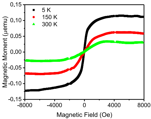
Fig. 4. Magnetisation versus magnetic field for the heat-treated sample (denotated as sample S2 in the main article).
