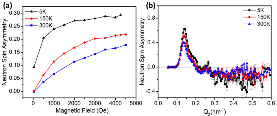
Fig. 5. (a) Magnetic field dependency of the neutron spin asymmetry, (b) Temperature dependency of the neutron spin asymmetry for the multi-energy implanted sample (denotated as sample S2 in the main article).
