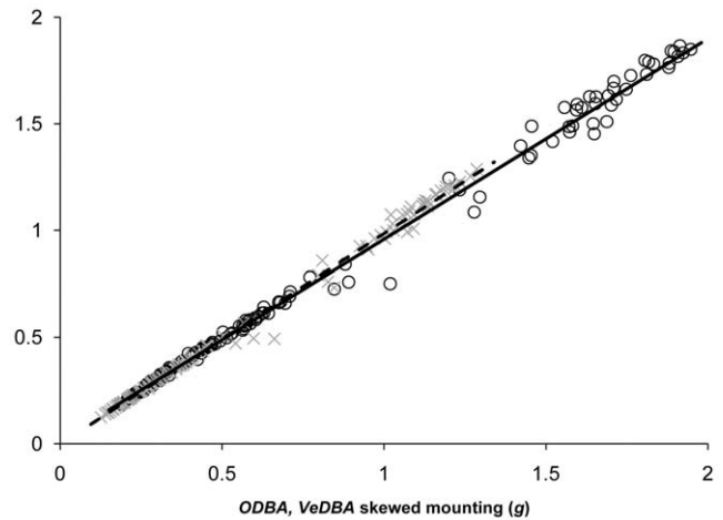
Figure 4. Dynamic body accelerations (ODBA – circles, and VeDBA – crosses) from straight- versus skew-mounted accelerometers (for details see text). Each point denotes a mean value derived from a three-minute trial of a participant moving at one particular speed below the lactate threshold. Data from all participants are included. doi:10.1371/journal.pone.0031187.g004
