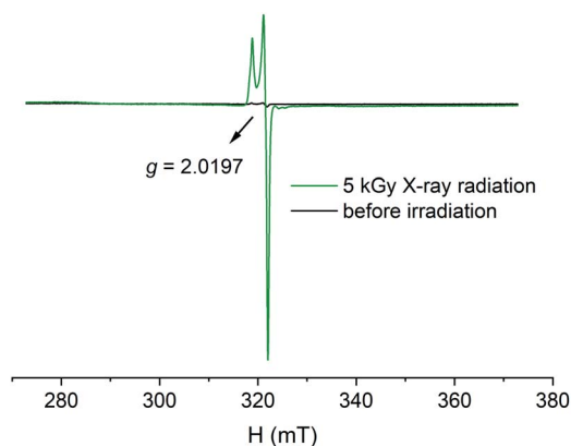
Fig. 3 EPR spectra of U-Cbdcp before and after 5 kGy X-ray irradiation.
