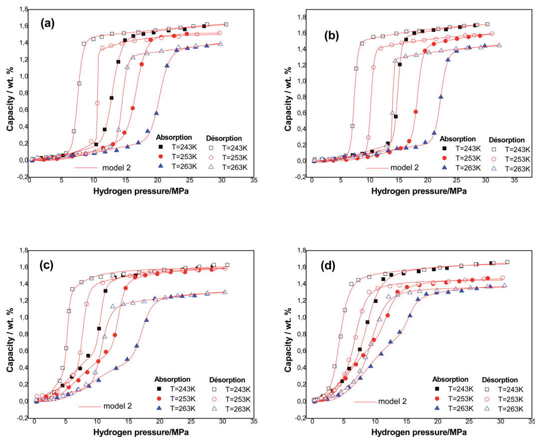
Fig. 3 Experimental absorption/desorption isotherms of hydrogen (dots) fitted by statistical model (continuous lines) at various temperatures of Ti_{1.02}Cr_{1.1}Mn_{0.3}Fe_{0.6}RE_{0.03} alloys: (a) Ti_{1.02}Cr_{1.1}Mn_{0.3}Fe_{0.6} alloy (b) Ti_{1.02}Cr_{1.1}Mn_{0.3}Fe_{0.6}La_{0.03} alloy; (c) Ti_{1.02}Cr_{1.1}Mn_{0.3}Fe_{0.6}Ce_{0.03} alloy; (d) Ti_{1.02}Cr_{1.1}Mn_{0.3}Fe_{0.6}Ho_{0.03} alloy.
