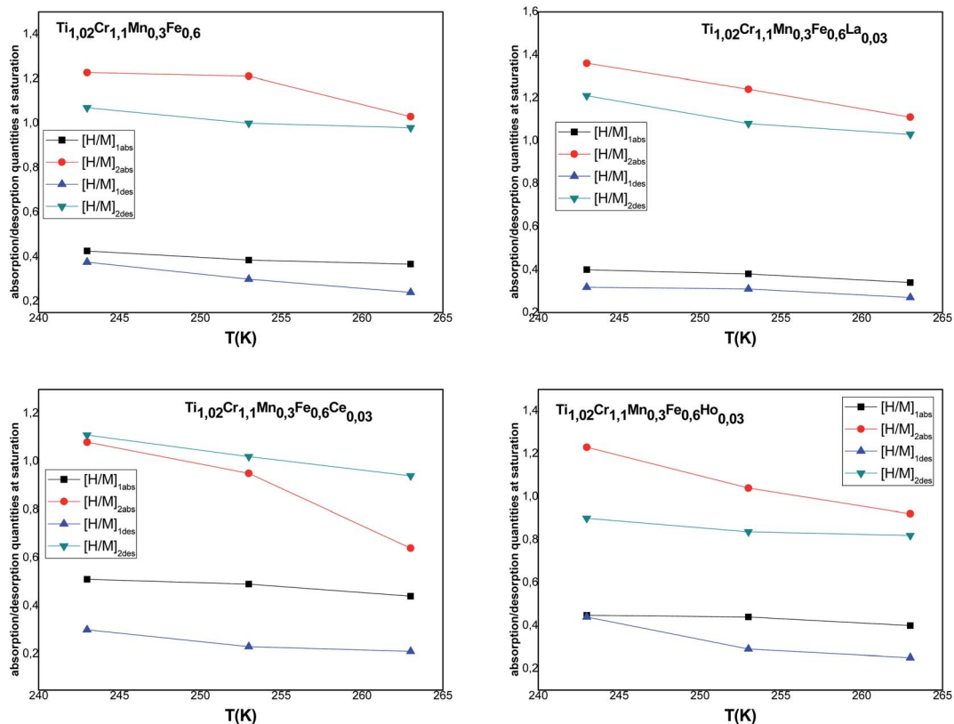
Fig. 6 Evolution of the monolayer absorbed/released quantities according to the temperature.
