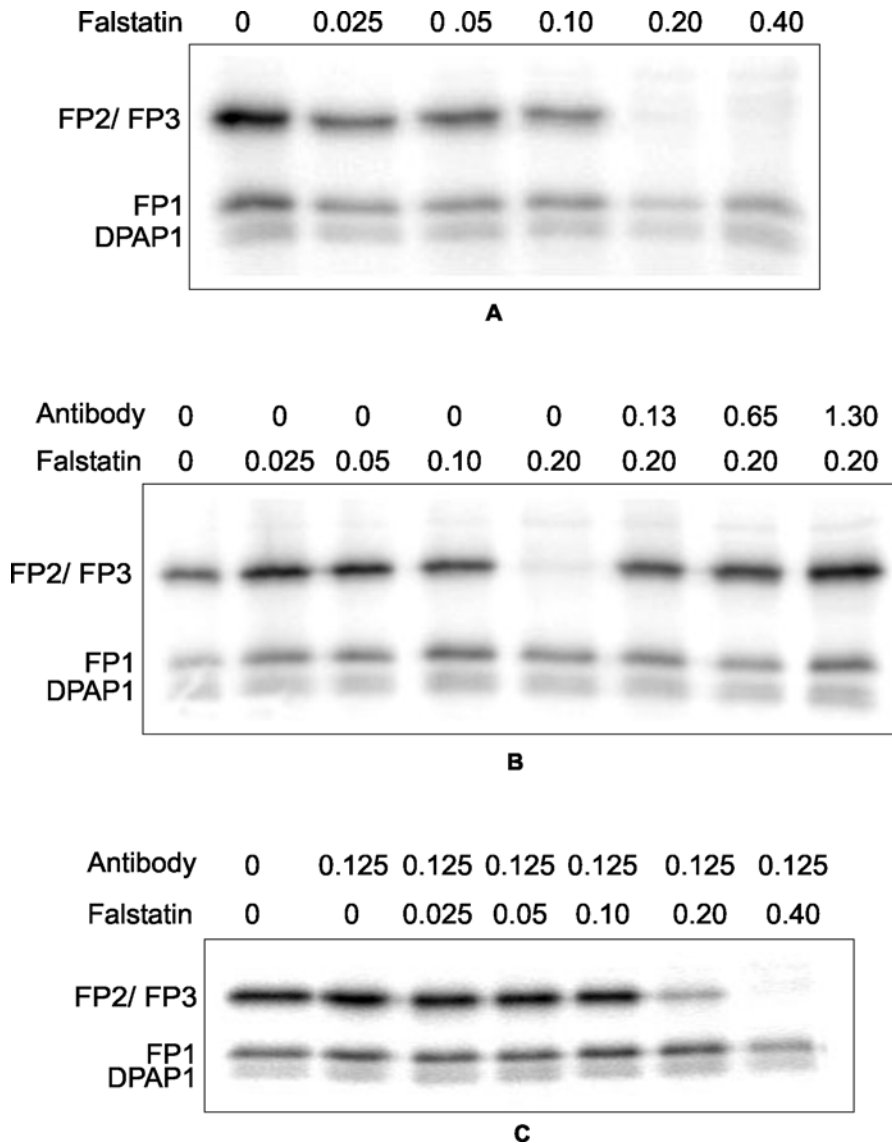
Figure 8. Inhibitor Competition
