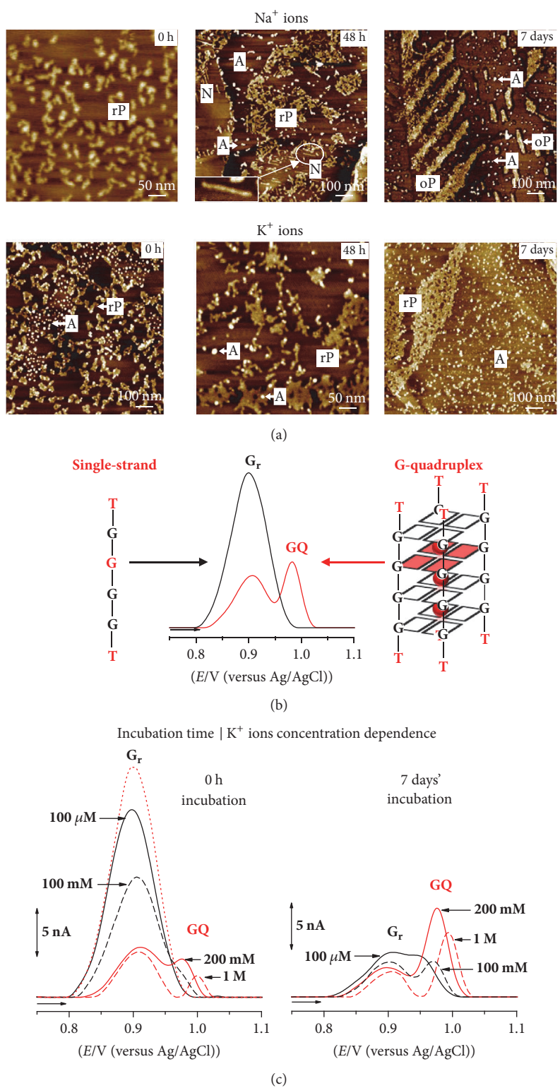
FIGURE 3: (a) AFM image of 0.3 \mu M d(TG_4T) in pH 7.0, in the presence of Na^+ and K^+ ions, at different incubation times; (b) representation of the d(TG_4T) single-strand and GQ electrochemical detection; (c) DP voltammograms baseline corrected in 3.0 \mu M d(TG_4T) in pH 7.0: incubation time and K^+ ions concentration dependence. [Adapted from [51] with permission.]
