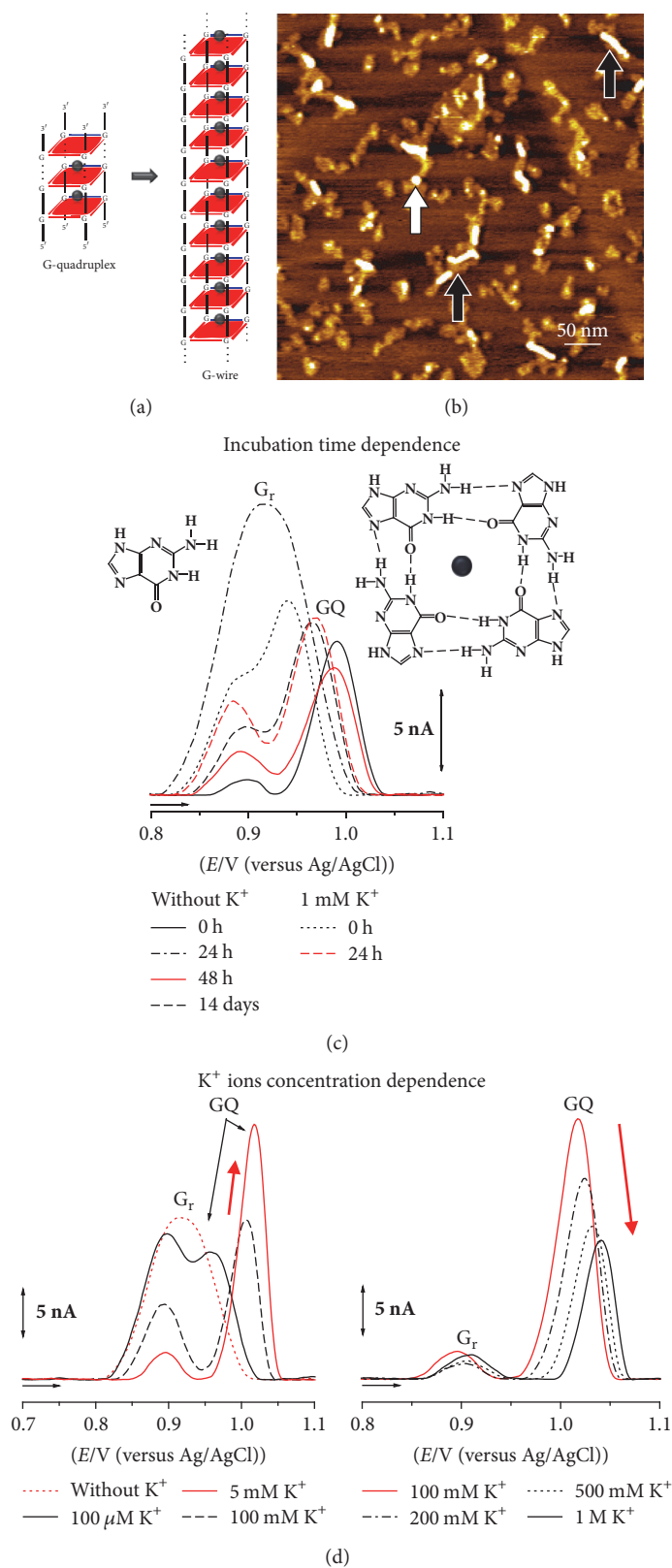
FIGURE 2: (a) Representation of d(G) 10 -GQ and GQ-based nanowire; (b) AFM image of 0.3 μM d(G) 10 in pH 7.0, 100 mM K + ions, at 24 h incubation; (c, d) DP voltammograms baseline corrected in 3.0 μM d(G) 10 in pH 7.0: (c) incubation time dependence and (d) K + ions concentration dependence at 0 h incubation. [Adapted from [50] with permission.]
