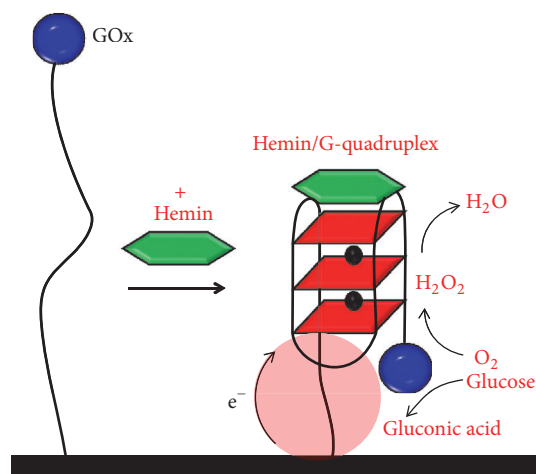
SCHEME 7: Hemin/G-quadruplex DNAzyme electrochemical biosensor for the detection of glucose.
