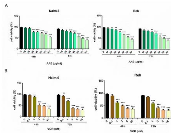
Figure 1. (A) Effect of individual treatment of AAE (10 to 90 \mu\text{g}/\text{ml} ) on Nalm-6 and Reh cells after 48 h and 72 h (B) Effect of individual treatment of VCR (0.1 to 10 nM) on Nalm-6 and Reh cells after 48 h and 72 h. The cell viability was determined by MTT assay. Each bar represents the mean \pm SD (n=3). *P< 0.05, **P< 0.01, ***P< 0.001 vs control; a P< 0.05, c P<0.001 vs VCR (one-way ANOVA and post hoc Tukey multiple comparison test).
