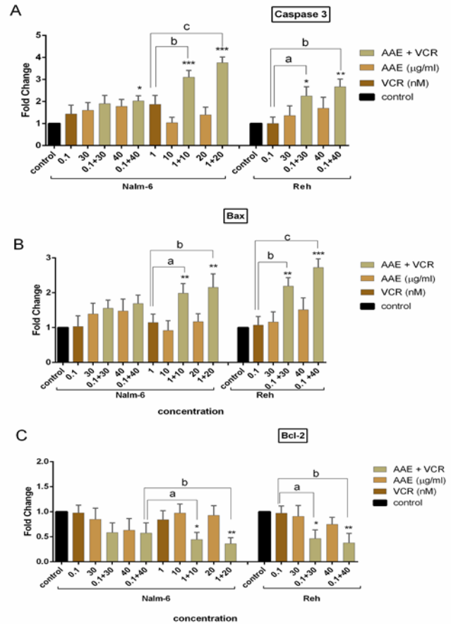
Figure 5. Quantitative real time-PCR analysis of (A) caspase 3, (B) Bax, (C) Bcl-2 mRNA expression levels in Nalm-6 and Reh cells. Total mRNA was detected by Real-time Quantitative PCR analysis. ABL served as an internal control. Each bar represents the mean ± SD (n=3). *P< 0.05, **P< 0.01, ***P< 0.001 vs control; †P <0.05, ††P< 0.01, †††P< 0.001 vs VCR (one-way ANOVA and post hoc Tukey multiple comparison test).
