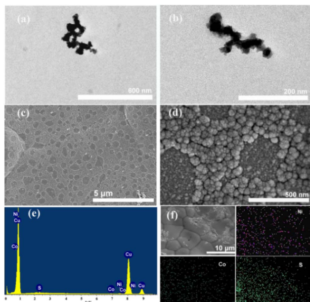
Fig. 2 TEM and SEM images and EDS of the CoNiS/CF electrode at (a) 600 nm scale, (b) 200 nm scale, (c) 5 \mu\text{m} scale, (d) 500 nm scale. (e) EDS spectrum, and (f) EDS mapping images of Ni, Co, S in scanned area.
