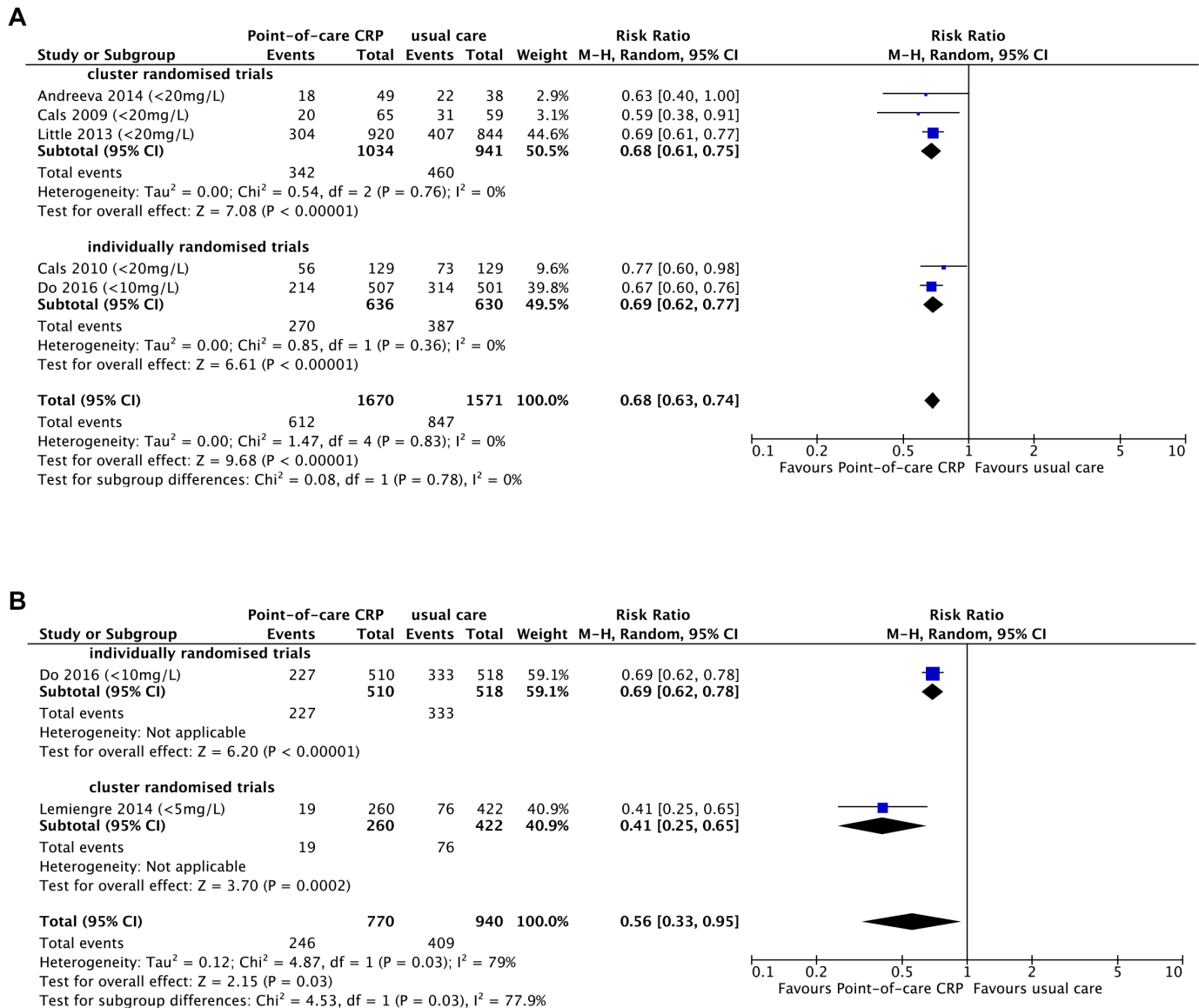
Figure 2 Forest plot of comparison: point-of-care CRP versus usual care, outcome: antibiotic prescribing at index consultation: (A) RCTs, adults only, if cut-off guidance applied; (B) RCTs, children only, if cut-off guidance applied. CRP cut-off used to withhold antibiotic treatment between brackets. CRP, C reactive protein; M-H, Mantel-Haenszel; RCTs, randomised controlled trials.
