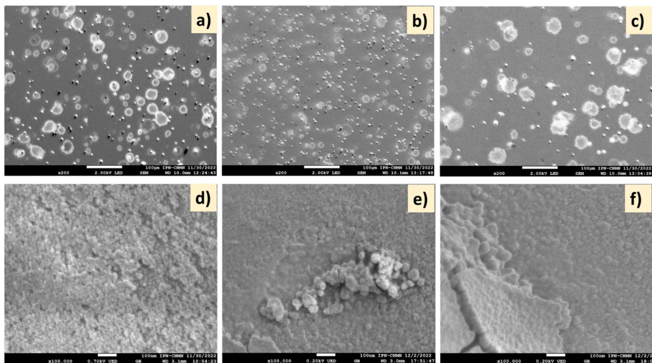
Fig. 3 SEM images of (a and d) CeH1T1, (b and e) CeH2T1, and (c and f) CeH2T2. Scale bars: (a–c) 100 μm and (d–f) 100 nm.
