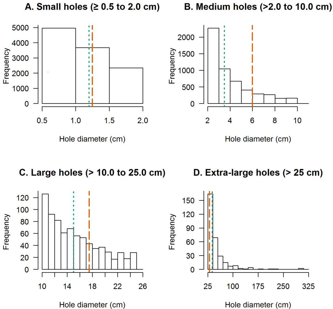
Fig 2. Histogram of measured hole diameters for each assigned WHOPEs hole category. The midpoint hole diameter used for the WHOPEs category weight is indicated by an orange dashed vertical line. The median hole diameter in each category is indicated by a green dotted vertical line.
