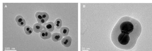
Fig. 3 TEM image of the purified SERS silica particles (A) using a low magnification, (B) using a high magnification.
