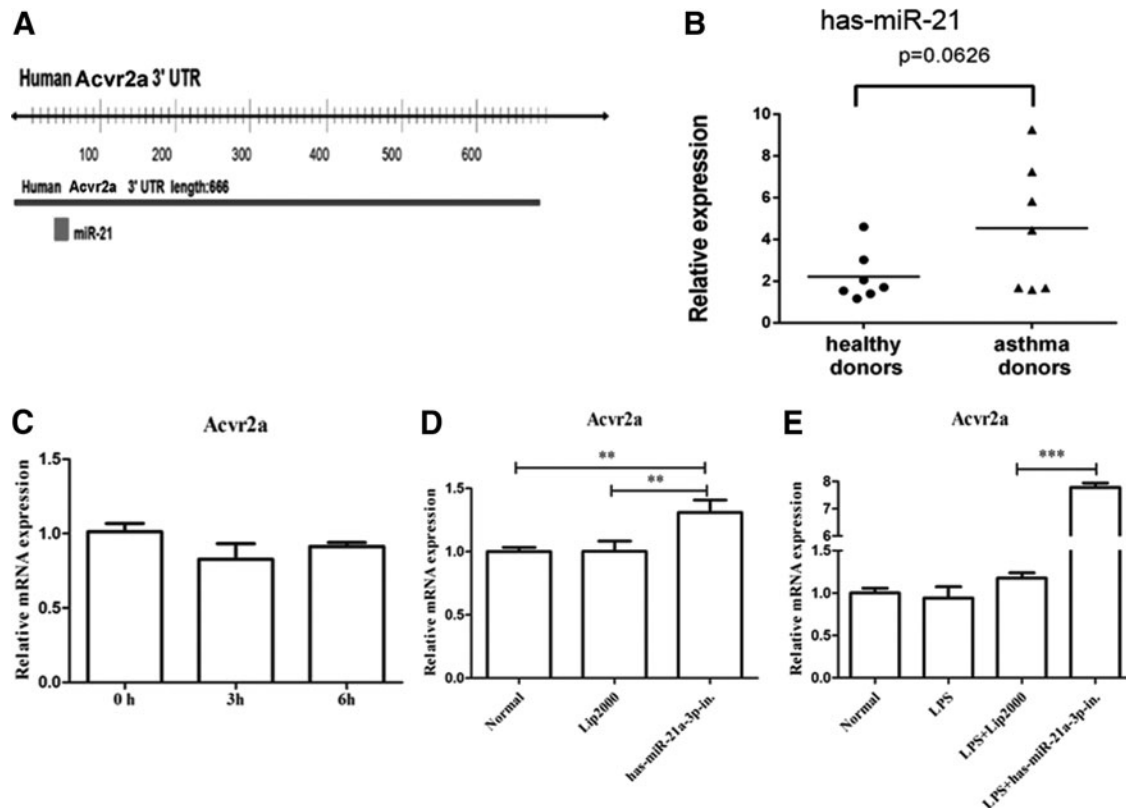
FIG. 6. Has-miR-21 regulates human Acvr2a expression. (A) The schematics show the interaction site for has-miR-21 that is harbored in the 3' UTR of the human Acvr2a mRNA transcript. (B) The mRNA expression levels of human has-miR-21 in asthma patients are shown. The has-miR-21 expression levels increased; however, they were not significantly different between the human bronchial epithelial cells from the asthmatic donors compared with the healthy donors. The has-miR-21 expression data were collected from NCBI Gene Expression Omnibus (GEO; GEO No. GSE25230). (C) BEAS-2B cells were cultured in indicated condition and exposed to 500 ng/mL LPS for 0, 3, and 6 h, respectively. (D) BEAS-2B cells were transfected with or without 500 pmol has-miR-21a inhibitor and cultured for 24 h. Lip 2000 group served as control. (E) BEAS-2B cells were transfected with or without 500 pmol has-miR-21a inhibitor for 24 h and then exposed to 500 ng/mL LPS for 3 h. Acvr2a mRNA levels were analyzed by qRT-PCR for (C–E). ** P < 0.01 ; *** P < 0.001 . LPS, lipopolysaccharide.
