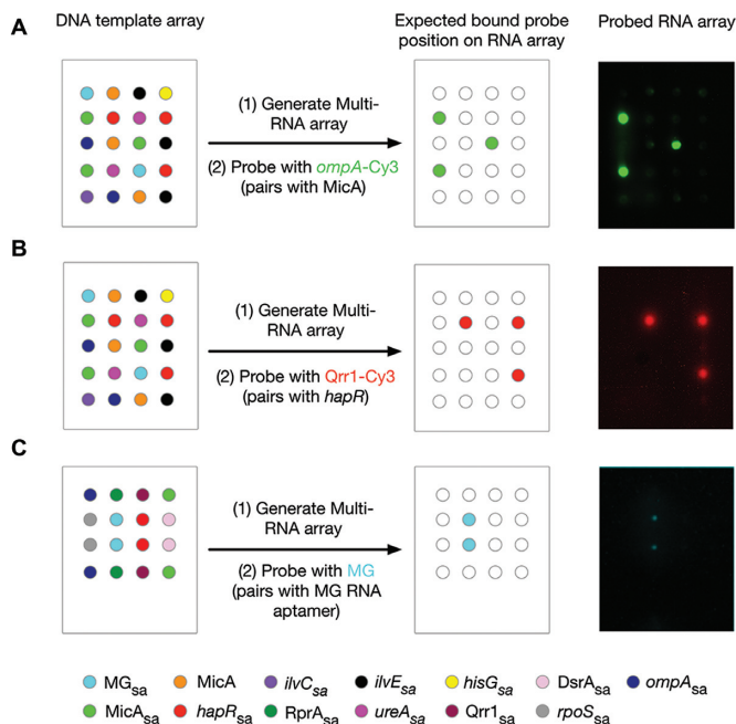
Figure 5. Production and screening of high-density multi-RNA arrays with single probes. (A) A DNA template array of MicA_{sa} , MicA , ompA_{sa} , hapR_{sa} , ilvC_{sa} , ilvE_{sa} , hisG_{sa} , ureA_{sa} and MG_{sa} templates (left: schematic of a single-field) was used to generate an eight-RNA array of MicA_{sa} , ompA_{sa} , hapR_{sa} , ilvC_{sa} , ilvE_{sa} , hisG_{sa} , ureA_{sa} and MG_{sa} that was probed with 3 \mu\text{M} Cy3-labelled ompA (right). (B) A DNA template array of MicA_{sa} , MicA , ompA_{sa} , hapR_{sa} , ilvC_{sa} , ilvE_{sa} , hisG_{sa} , ureA_{sa} and MG_{sa} templates (left: schematic of a single-field) was used to generate an eight-RNA array of MicA_{sa} , ompA_{sa} , hapR_{sa} , ilvC_{sa} , ilvE_{sa} , hisG_{sa} , ureA_{sa} and MG_{sa} that was probed with 2.5 \mu\text{M} Cy3-labelled Qrr1 (right). The probed array has been false-coloured red to match the key. (C) A DNA template array of MicA_{sa} , Qrr1_{sa} , DsrA_{sa} , RprA_{sa} , hapR_{sa} , ompA_{sa} , rpoS_{sa} and MG_{sa} templates (left: schematic of a single-field) was used to generate an eight-RNA array of MicA_{sa} , Qrr1_{sa} , DsrA_{sa} , RprA_{sa} , hapR_{sa} , ompA_{sa} , rpoS_{sa} and MG_{sa} that was probed with 20 \mu\text{M} malachite green (right). The probed array has been false-coloured cyan to match the key. DNA template arrays of repeating 4 \times 5 grids (A and B) or 4 \times 4 grids (C) were prepared using an automated arrayer with individual spots separated by 1250 \mu\text{m} . Probed RNA images have all been mirror imaged so that the spot positions correspond to those shown in the schematic of the DNA template arrays.
