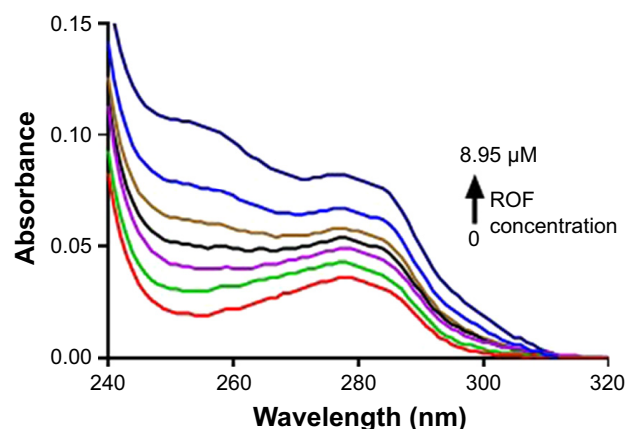
Figure 4 Spectra for UV absorption of BSA (1.5 \mu M) and BSA in presence of ROF at room temperature.
