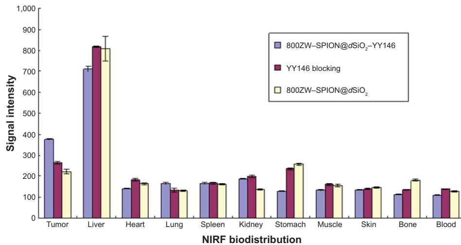
Figure 7 Biodistribution analysis.
