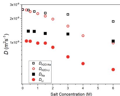
Fig. 1 Concentration-dependent diffusion constants for {}^7\text{Li} ( D_{\text{Li}} ), {}^{23}\text{Na} ( D_{\text{Na}} ), and {}^1\text{H} (solvent \text{H}_2\text{O} , D_{\text{H}_2\text{O}-\text{Li}} and D_{\text{H}_2\text{O}-\text{Na}} ) at 303 K in aqueous solutions.
