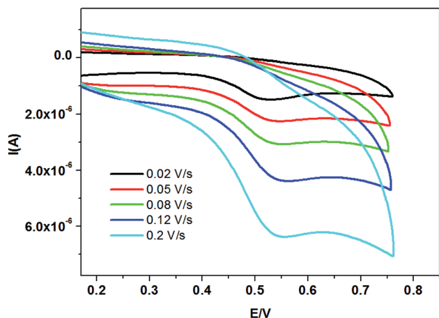
Fig. 7 Cyclic voltammograms of SH- \beta -CD-AuNPs-1/GO/GCE in 0.1 \mu M TBBPA at different scan rates.
