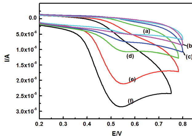
Fig. 4 Cyclic voltammograms of (a) bare GC, (b) GO/GCE, (c) AuNPs-1/GO/GCE, (d) SH-β-CD-AuNPs-3/GO/GCE, (e) SH-β-CD-AuNPs-2/GO/GCE, and (f) SH-β-CD-AuNPs-1/GO/GCE in 5 \times 10^{-7} mol L -1 TBBPA and PBS buffer solution (pH = 7.0).
