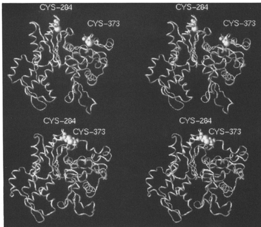
Figure 8. Computer modeling of ISC \beta -actin. Stereo view of the beta actin crystal structure backbone ( top ) with the profilin chaperon portion removed. In the crystal structure, the CYS 373 and 284 side chain sulfur atoms are 21.63 Å apart. The second model ( bottom ) represents \beta -actin with the disulfide bridge formed between residues CYS 373 and CYS 284.
