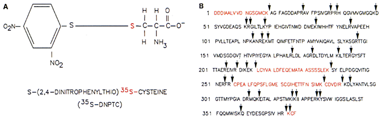
Figure 5. Structure of 35 S-DNPTC and \beta -actin. ( Left ) The structure of S-(2,4-dinitrophenylthio)[ 35 S]cysteine or 35 S-DNPTC is presented. The radioactive sulfur is shown in red. ( Right ) The primary structure of \beta -actin is presented using the single letter code for amino acids. The arrows indicate sites of trypsin cleavage. Stretches of amino acids in red indicate tryptic peptides which contain cysteine residues. K 372 is in red because under our conditions cleavage after K 372 occurs less frequently than cleavage after R 371 , therefore KCF is generated.
