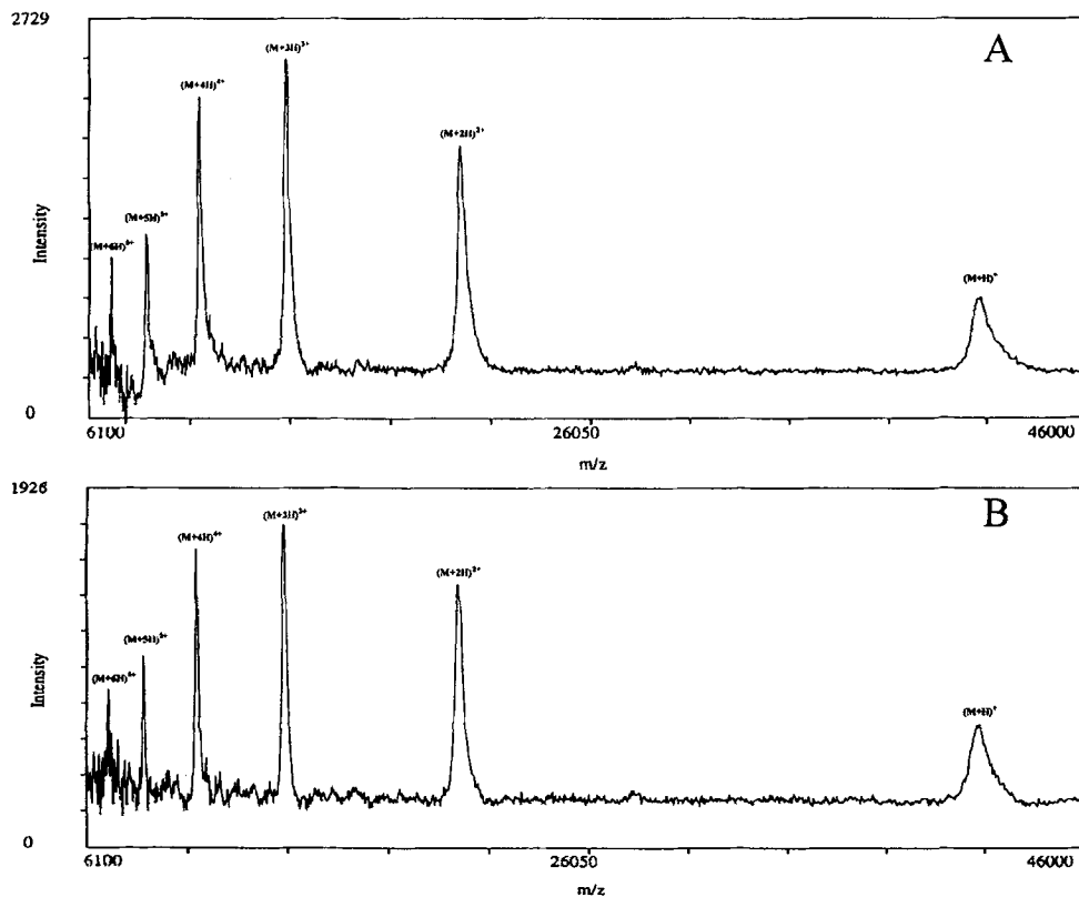
Figure 7. Molecular weight determination of \beta -actin from MALDI-TOF spectra. MALDI-TOF mass spectra of \beta -actin isolated from control AA erythrocytes (A) and HDSS erythrocytes (B). The molecular weights were 41,690 \pm 100 and 41,760 \pm 100 , respectively.
