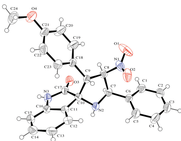
Figure 5 The molecular structure of compound (II) showing the atom numbering scheme. Displacement ellipsoids are drawn at the 40% probability level, using ORTEP-3. Hydrogen atoms are drawn as spheres of arbitrary size.
