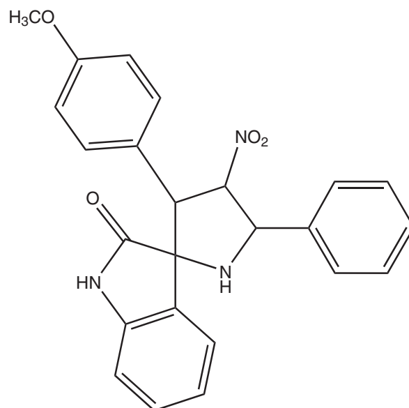
Scheme 3 Scheme showing the structural formula of compound (II).
