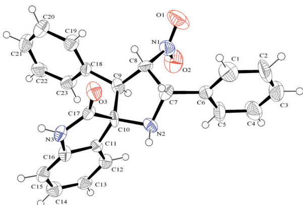
Figure 4 The molecular structure of compound (I) showing the atom numbering scheme. Displacement ellipsoids are drawn at the 40% probability level, using ORTEP-3. Hydrogen atoms are drawn as spheres of arbitrary size.
