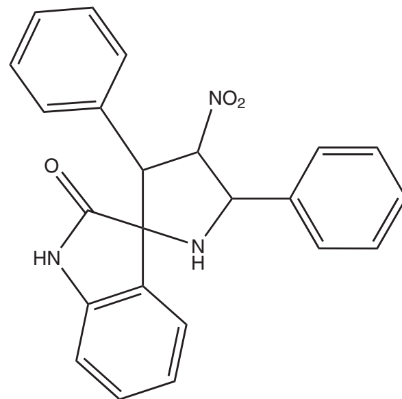
Scheme 2 Scheme showing the structural formula of compound (I).
