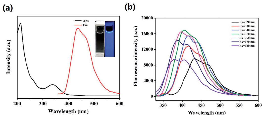
Fig. 3 (a) UV-Vis absorption spectrum and fluorescence spectrums ( \lambda_{\text{ex}} = 350 \text{ nm} ) (inset: photographs of HS-CQDs under the radiation of (left) visible light and (right) 365 nm UV light). (b) Fluorescence spectra of HS-CQDs solutions ( 25 \mu\text{g mL}^{-1} ) with different excitation wavelengths from 320 nm to 380 nm.
