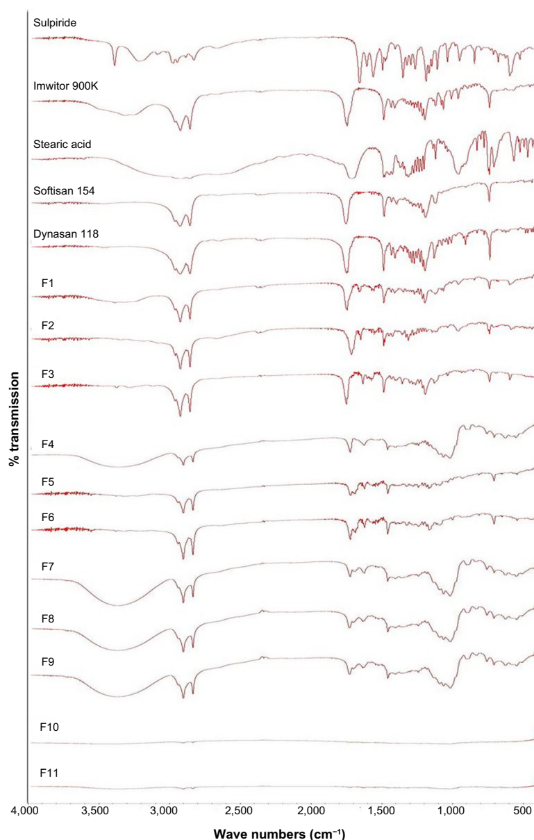
Figure 5 Fourier transform infrared spectra for sulphiride, Imwitor ® 900K, stearic acid, Softisan ® 154, Dynasan ® 118, and solid lipid nanoparticle formulations (F1–F11). Note: Imwitor ® 900K, Softisan ® 154, and Dynasan ® 118 all from Sasol Germany GmbH (Witten, Germany).
