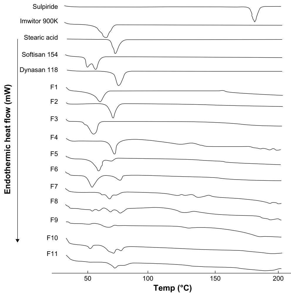
Figure 4 Differential scanning calorimetric thermograms for sulphiride, Imwitor® 900K, stearic acid, Softisan® 154, Dynasan® 118, and solid lipid nanoparticle formulations (F1–F11). Note: Imwitor® 900K, Softisan® 154, and Dynasan® 118 all from Sasol Germany GmbH (Witten, Germany).
