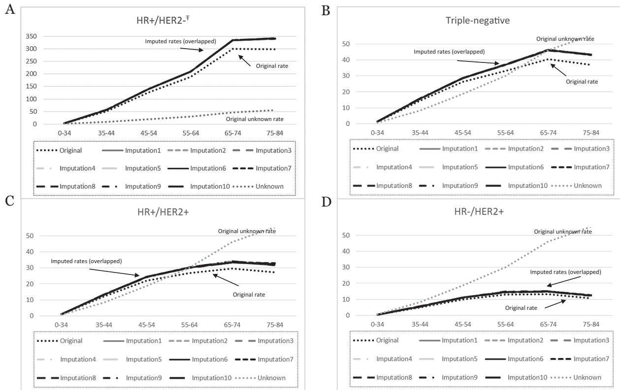
Figure 1. Original vs imputed age-specific rates by subtype, unknown subtype for diagnosis year 2011, and areas in the United States with high-quality incidence data *,^ . A) Hormone receptor (HR+)/ human epidermal growth factor receptor 2 (HER2)- rates per 100 000 women † . B) Triple-negative rates per 100 000 women. C) HR+/HER2+ rates per 100 000 women. D) HR-/HER2+ rates per 100 000 women. *Population-based registries meeting North American Association of Central Cancer Registries quality criteria and high completeness of HR/HER2 data include: Alaska, California, Colorado, Connecticut, Delaware, District of Columbia, Florida, Georgia, Hawai'i, Idaho, Illinois, Indiana, Iowa, Kansas, Kentucky, Louisiana, Maine, Maryland, Massachusetts, Michigan, Mississippi, Missouri, Montana, Nebraska, New Hampshire, New Jersey, New Mexico, New York, North Carolina, North Dakota, Ohio, Oregon, Pennsylvania, Rhode Island, South Carolina, South Dakota, Utah, Vermont, Virginia, Washington, West Virginia, Wisconsin, Wyoming. ^All 10 imputations had near identical rate estimates. †Note: HR+/HER2- has much higher rates, so this figure has a different y-axis. The unknown rate is a reference rate from the original data and is the same for each figure. HER2 = human epidermal growth factor receptor 2; HR = hormone receptor.
