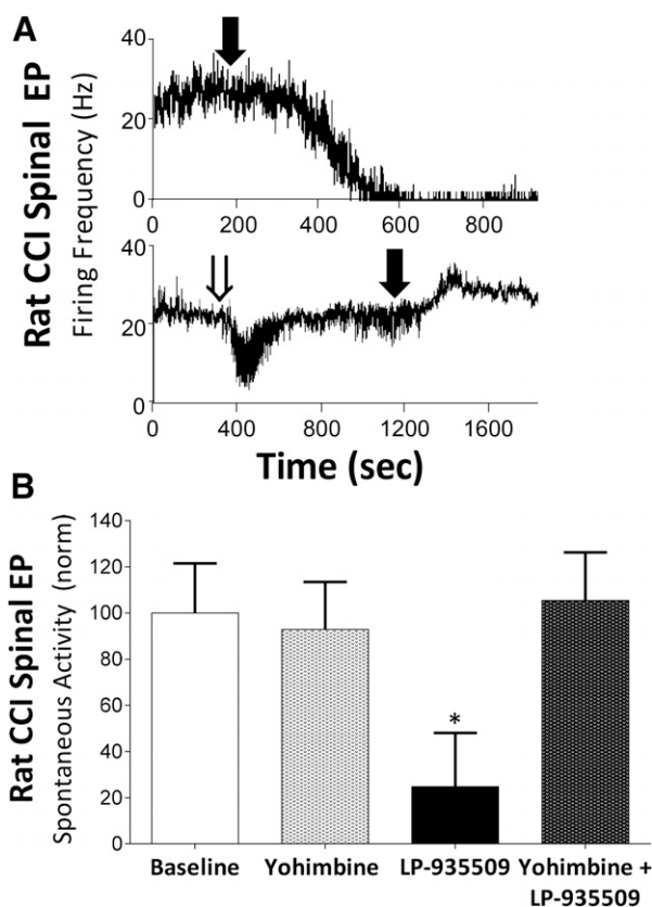
Fig. 10. \alpha 2 adrenergic antagonist blocks AAK1 inhibition-induced reduction in spontaneous neuronal activity in CCI rats. (A) CCI rat spontaneous activity time course of two individual spinal dorsal horn neurons treated with LP-935509 (1 mg/kg, i.v.; filled arrow) without (top trace) or with (bottom trace) pretreatment of yohimbine (0.3 mg/kg, i.v.; open arrow). (B) CCI rat group data for spontaneous activity with design and dosing as in (A) plus baseline and yohimbine controls ( n = 6-8 male rats per group). * P < 0.05 versus baseline by one-way analysis of variance, followed by Dunnett's t test.
