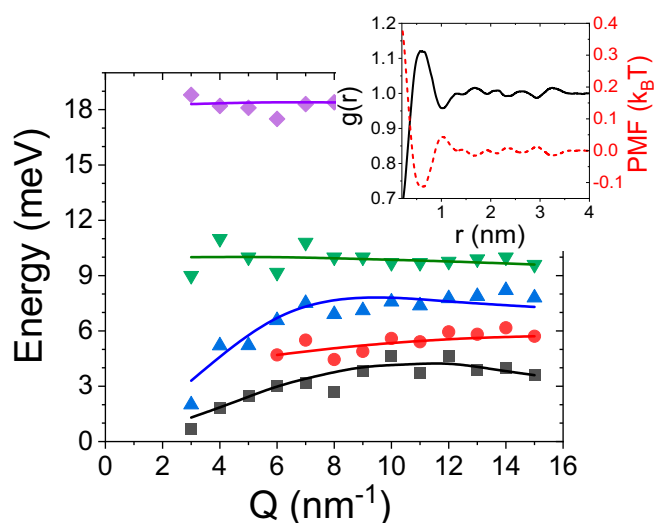
Fig. 5. Dispersion curves obtained using the modeling of the longitudinal current correlation spectra, C_L(Q, E) , calculated by MD simulation for the system containing 30\% Chol at 25 \text{ }^\circ\text{C} . The detailed description of the modeling procedure of C_L(Q, E) spectra can be found elsewhere (42). Inset shows the lateral radial pair distribution function g(r) for DPPC-Chol pairs and the corresponding potential of mean force, \text{PMF}(r) , calculated according to \text{PMF}(r) = -k_B T \ln g(r) .
