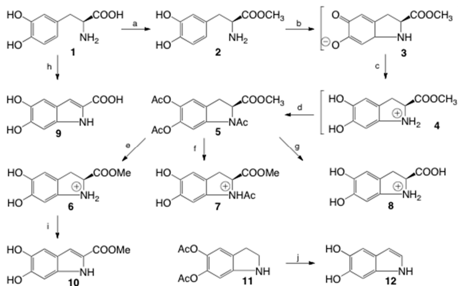
Figure 1. Synthetic scheme for the preparation of cycloDOPA derivatives. (a) SOCl_2 , MeOH, reflux, 1h, quant; (b) K_3[Fe(CN)_6] , sodium phosphate (pH = 8), 0 °C, 75 s; (c) Na_2S_2O_4 , sodium phosphate (pH 8), 0 °C, 30 s; (d) Ac_2O , pyridine, rt, 4 h, 60% (3 steps); (e) AcCl , MeOH, 60 °C, 16 h, 97%; (f) 1 M HCl, MeOH, rt, 3 days, 59%; (g) 6 M HCl, 80 °C, 5 h, 94%; (h) (1) K_3[Fe(CN)_6] , NaHCO_3 , rt, 5 min, (2) 1M NaOH, rt, 15 min, 71%; (i) NaOH (pH = 10), rt, o/n, 48%, (j) K_2CO_3 , MeOH, 0 °C, 50 min, 51%.
