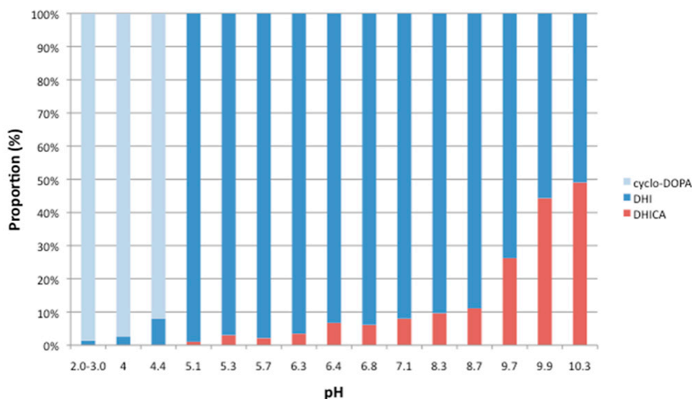
Figure 3. The products distributions of the decomposition of cycloDOPA ( 8 ) at different pH levels. CycloDOPA ( 8 , 35 mg) was dissolved in D 2 O (0.5 mL) and CH 3 CN (1 μL), and the solution was adjusted to the indicated pH with a NaOD solution. The incubation time refers to the time required for cycloDOPA to be consumed completely, expected pH = 3.6 and pH = 4.4.
