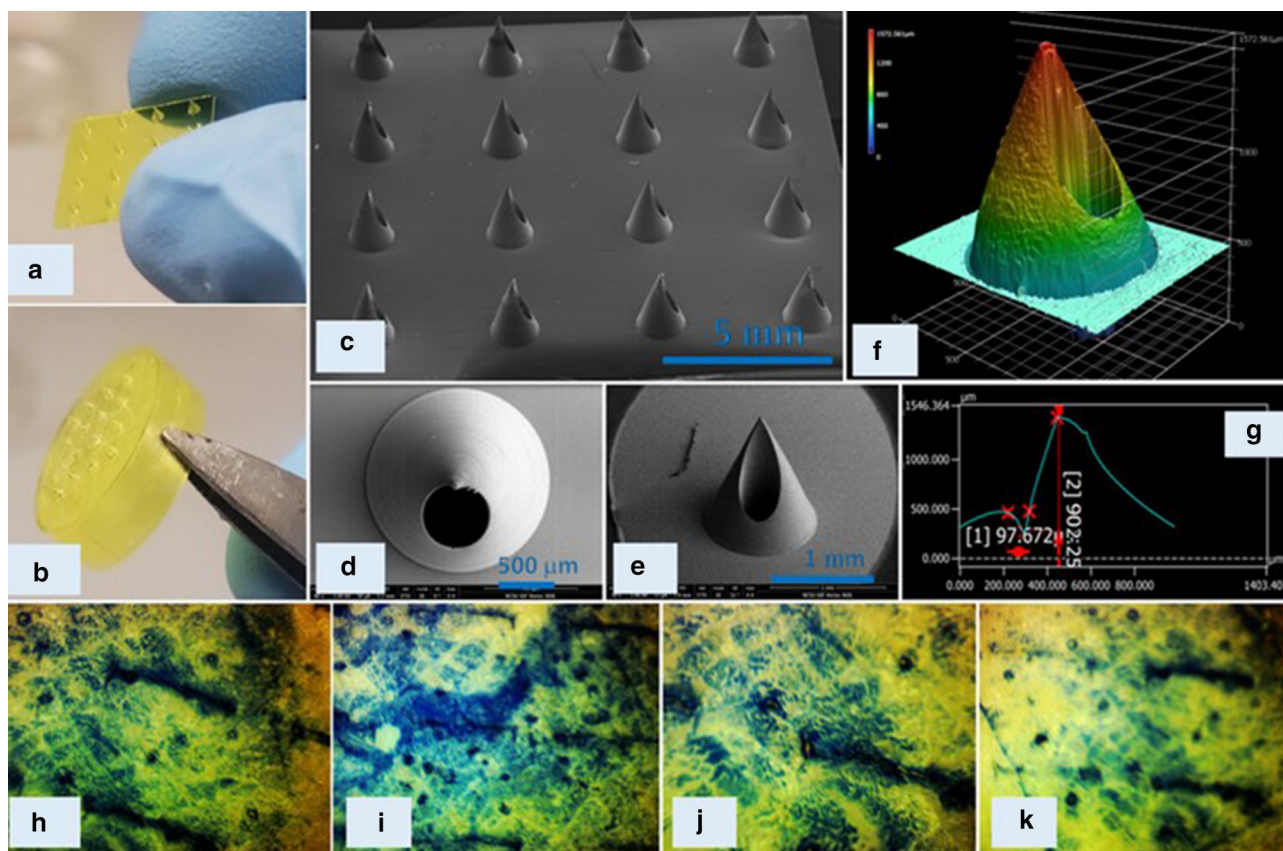
Figure 6. The hollow MN array component of a point-of-care system. Optical images of MN arrays on (a) a square plate and (b) a cap. SEM images of (c) an MN array, (d) an MN tip, and (e) an MN (oblique view). Keyence laser scanning optical microscopy 3D images of the (f) MN and (g) dimensions of the MN as indicated by the plot of the height (y-axis) and width of the needle (x-axis). Optical images of trypan blue-coated punctured porcine skin using MN arrays of height of (h) 750 \mu\text{m} , (i) 800 \mu\text{m} , (j) 900 \mu\text{m} , and (k) 950 \mu\text{m} . Trypan blue was applied to the MN array-treated skin for visualization of the MN array-generated pores as shown in Figure 3h–k. The MN arrays were inserted into the skin through manual application. The MN array penetrated the stratum corneum layer of the porcine skin without damage to the MN tips (Shukla et al., 2023). 3D, three-dimensional; MN, microneedle; SEM, scanning electron microscope.
