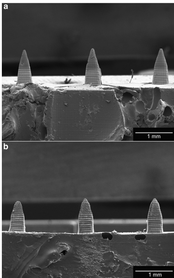
Figure 4. Scanning electron micrographs of unmodified and quantum-dot coated Gantrez microneedles. The micrographs show (a) unmodified Gantrez microneedles and (b) quantum-dot coated Gantrez microneedles, which were produced using visible light dynamic mask microstereolithography-micromolding and piezoelectric inkjet printing. This image was reprinted with permission from Boehm et al. (2011).
