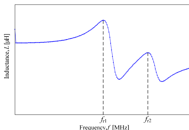
Figure 5. Expected dual resonant frequencies.
