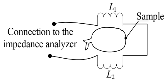
Figure 4. Electrical diagram for the dual flat type shape air coil.
