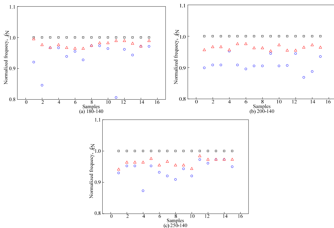
Figure 8. Normalized resonant frequency of the first peak for each coil's turns configuration. \square air \triangle ripe \circ unripe.
