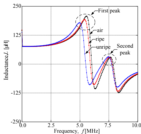
Figure 7. Inductance characteristics of the oil palm fruit sensor.
