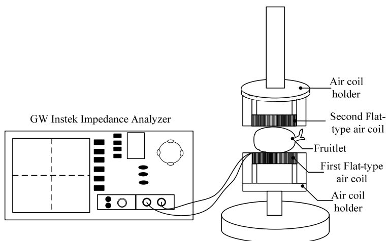
Figure 3. Samples preparation for the dual flat-type shape air coil. (a) Experimental setup, (b) Sample close up.
