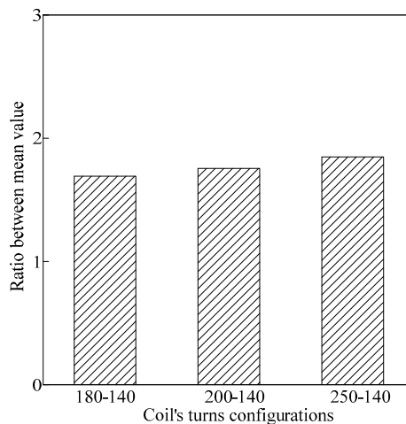
Figure 13. Ratio between \delta_{unripe} and \delta_{ripe} for each coil turn configuration.
