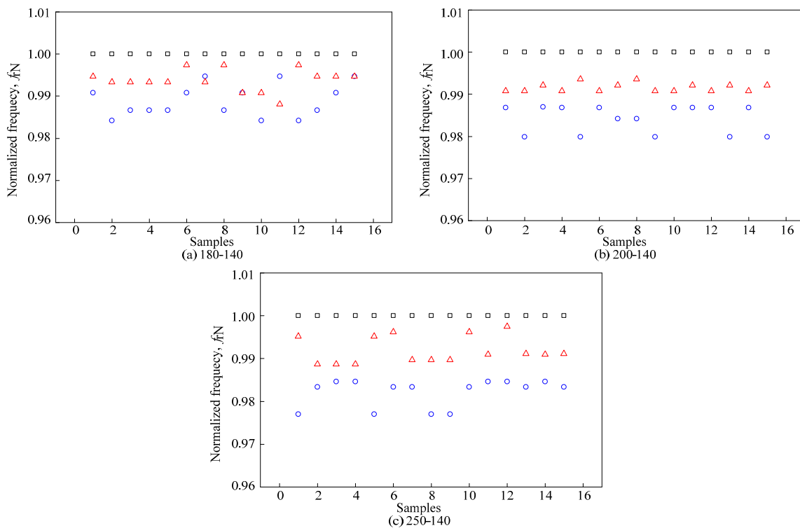
Figure 11. Normalized resonant frequency of the second peak for each coil’s turns configuration: \square air \triangle ripe \circ unripe.
