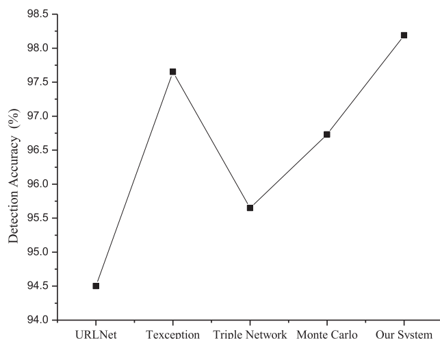
Fig. 13. Comparison of Detection Accuracies with State-of-art detection methods.
