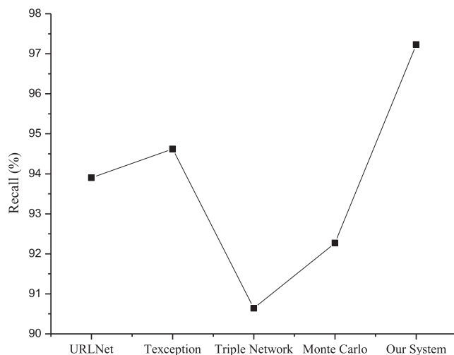
Fig. 14. Comparison of Recall with State-of-art detection methods.
