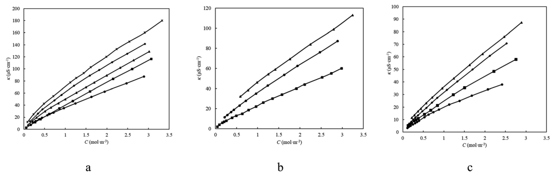
Fig. 1 Specific conductivity ( \kappa ) of, (a) [BHEA][Lau] in aqueous solutions at; ● 298.15 K, ■ 303.15 K, ◆ 308.15 K, ▲ 313.15 K, * at 318.15 K, temperatures. (b) SAILs in aqueous solutions at 298.15 K; ▲ [2-HEA][Lau], ● [BHEA][Lau], ■ [THEA][Lau]. (c) [BHEA][Lau] in aqueous gabapentin solutions with different molality concentration of gabapentin ( \text{mol kg}^{-1} ); ▲, 0.0000, ◆, 0.0100, ■, 0.0300, ● 0.0500 at 298.15 K.
