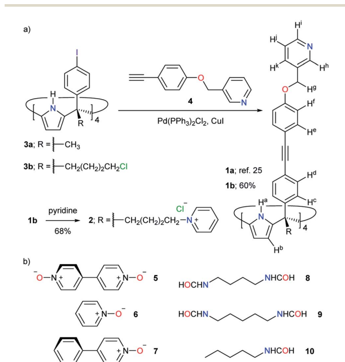
Fig. 2 (a) Synthesis of tetra-pyridyl SAE-ligands 1a , 1b and 2 . (b) Line-drawing structures of guests 5 – 10 used in this study.
