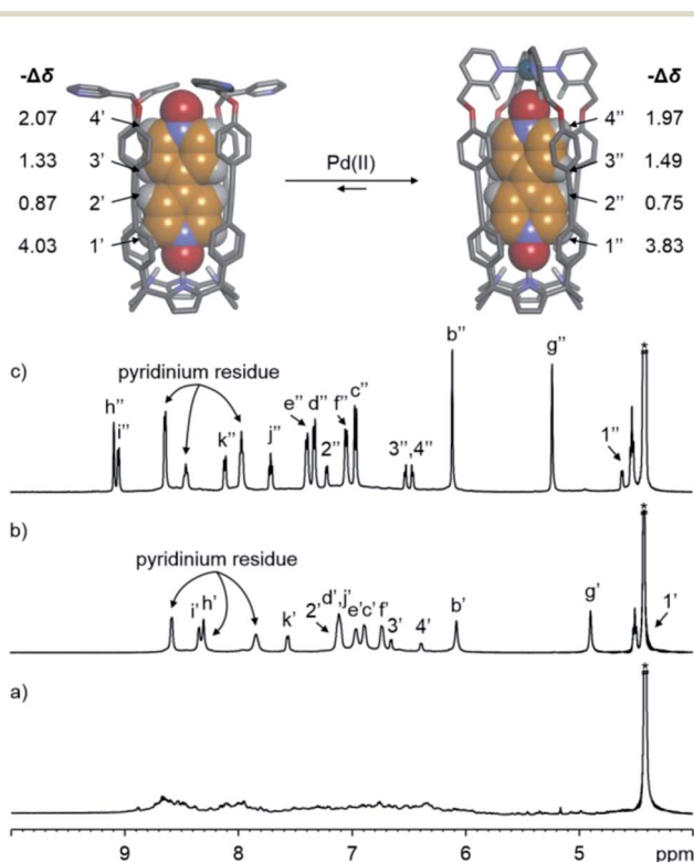
Fig. 4 (Top) Energy minimized structures (MM3) of the simplified 5 \subset 2^{4+} and 5 \subset [2 \cdot \text{Pd}]^{6+} inclusion complexes. (Bottom) Selected regions of the ^1\text{H} NMR (500 MHz with a cryoprobe, \text{D}_2\text{O} , 333 K) spectra of (a) 2^{4+} , (b) 5 \subset 2^{4+} and (c) 5 \subset [2 \cdot \text{Pd}]^{6+} . Primed and double primed labels correspond to the proton signals of 5 \subset 2^{4+} and 5 \subset [2 \cdot \text{Pd}]^{6+} , respectively. See Fig. 2a for the proton assignment of bound 2^{4+} . *Residual solvent peak.
