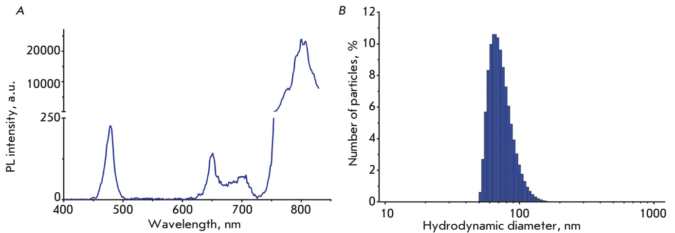
Fig. 1. Properties of \text{NaYF}_4:\text{Yb,Tm} UCNPs. A – PL emission spectra of the UCNPs excited by a 980-nm light; B – size distribution of the UCNPs with PMAO- and PEG-DGE-modified surface
