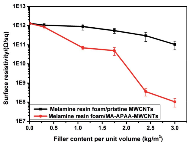
Fig. 9 Surface resistivity of melamine foam/pristine MWCNTs (a) and melamine foam/MA-APAA-MWCNTs (b) nanocomposite.
