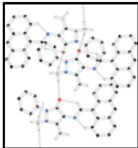
Fig. 2. Partial packing diagram showing connectivity between molecules (dashed lines). H atoms not involved in intermolecular interactions are omitted for clarity.
