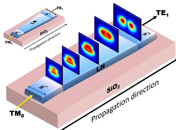
Figure 16. Mode profiles along the direction of propagation in Y-propagating LN taper for conversion from \text{TM}_0 to \text{TE}_1 mode. [Lumerical 2020a Finite Difference IDE, version: 8.23.2152, release: 2020a r2, URL: www.lumerical.com ] [Image converted to JPG file with Adobe Photoshop, Version: 21.2.1 20200716.r.265, URL: www.adobe.com ].
