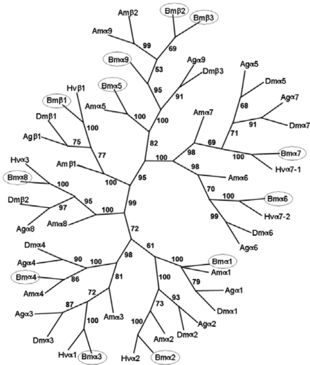
Figure 2 Phylogenetic relationship of insect nAChR subunits.
