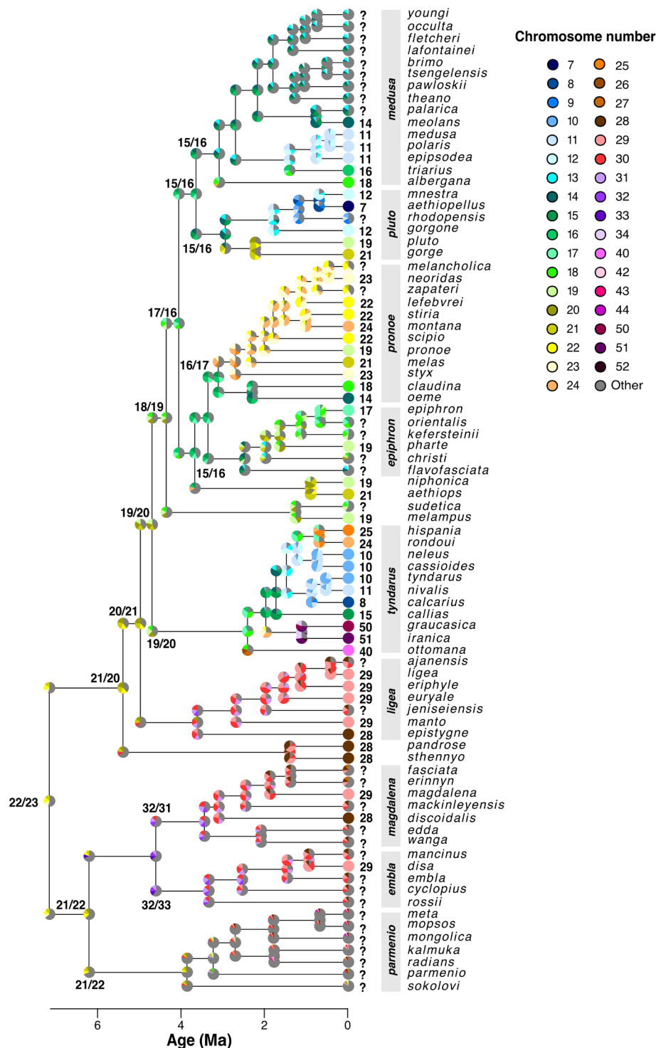
Fig. 2. Summary of the chromosome evolution model for Erebia , implemented in ChromoSSE. Estimated ancestral chromosome numbers for Erebia , inferred using the phylogenomic topology of fig. S1. Chromosome numbers are indicated proportionally by the color of the pie charts at the branch nodes. The pie charts at the “shoulders” of each node represent the inferred chromosomal state immediately after a speciation event. The two inferred chromosome numbers with highest posterior distribution of the ancestor of each clade are depicted atop or below the node that starts that clade. For deeper nodes within the tree, the reconstructed ancestral character states are likewise presented. For each extant species in the phylogeny, the karyotype is shown before the name. When the karyotype of a species is not known, the species is denoted with a “?”. Clades are named as in Fig. 1. The posterior probabilities of reconstructed ancestral chromosome states are visualized in fig. S7.
