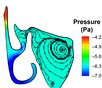
Figure 2 Airflow dynamics in the nasal-sinus airway.
