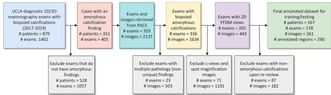
Fig. 1. Cohort selection.
