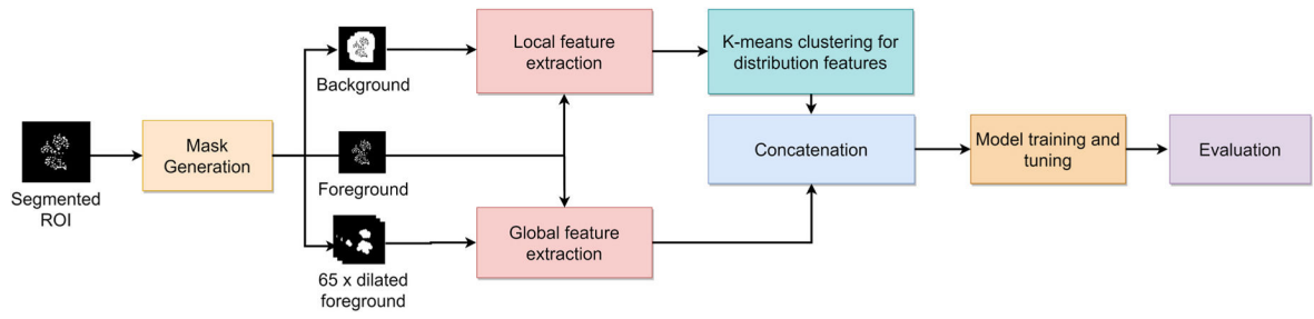
Fig. 2. Classification pipeline.
