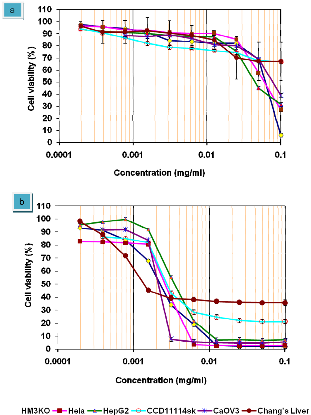
Figure 1 Dose-response curve of E. longifolia crude extract and Tamoxifen against malignant cells (HM3KO, Hela, HepG2 and CaOV3) and non-malignant cells (CCD1114sk and Chang's liver). E. longifolia crude extract showed a higher toxicity towards HepG2 cells compared to the other cell lines used in the experiment. Non-malignant cells, Chang's Liver and CCD1114sk were not significantly affected by the crude extract and no IC_{50} was evident (a). Tamoxifen showed a cytotoxic effects on all of the cell lines used in the experiment including non-malignant cells, Chang's liver and CCD1114sk (b). The values of graph represent mean \pm S.D of three independent experiments. P < 0.05 .
