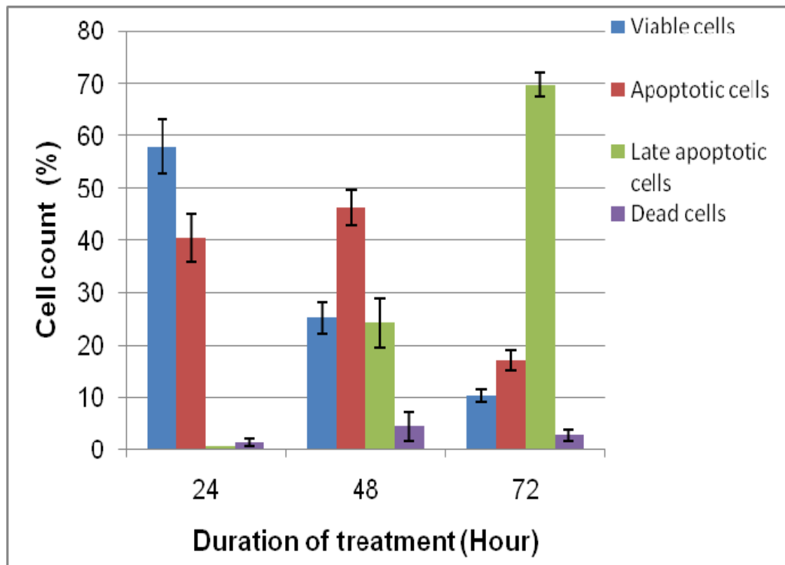
Figure 8 Scatter plots of Ann/PI-stained HepG2 cells treated-vinblastine sulfate (2.5 µg/ml) under four situations in quadrant analysis. They are living cells (A3), apoptotic cells (A4), late apoptotic or dead cells (A2) and necrotic or dead cells (A1). Exposed for 24 hours (1); exposed for 48 hours (2); exposed for 72 hours (3)(a). The graph summarized the numbers of cells in each quadrant (b). The values of the bars represented mean ± S.D. of three independent experiments. P < 0.05.
