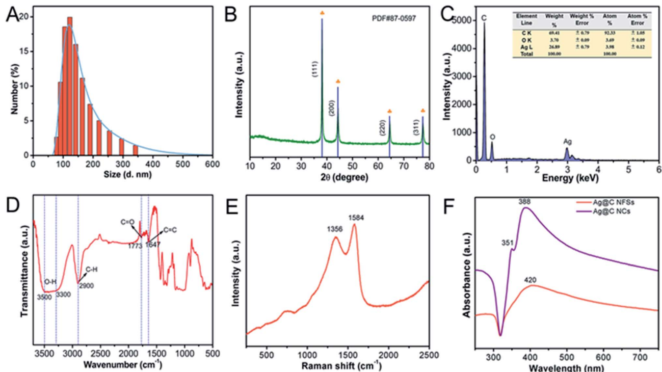
Fig. 3 (A) Hydrodynamic diameter of Ag@C NFSs. (B) XRD pattern of Ag@C NFSs. (C) The EDS of Ag@C NFSs. (D) FT-IR spectra of Ag@C NFSs. (E) Raman spectrum of Ag@C NFSs. (F) UV-vis absorbance spectra of Ag@C NFSs and Ag@C NCs.
