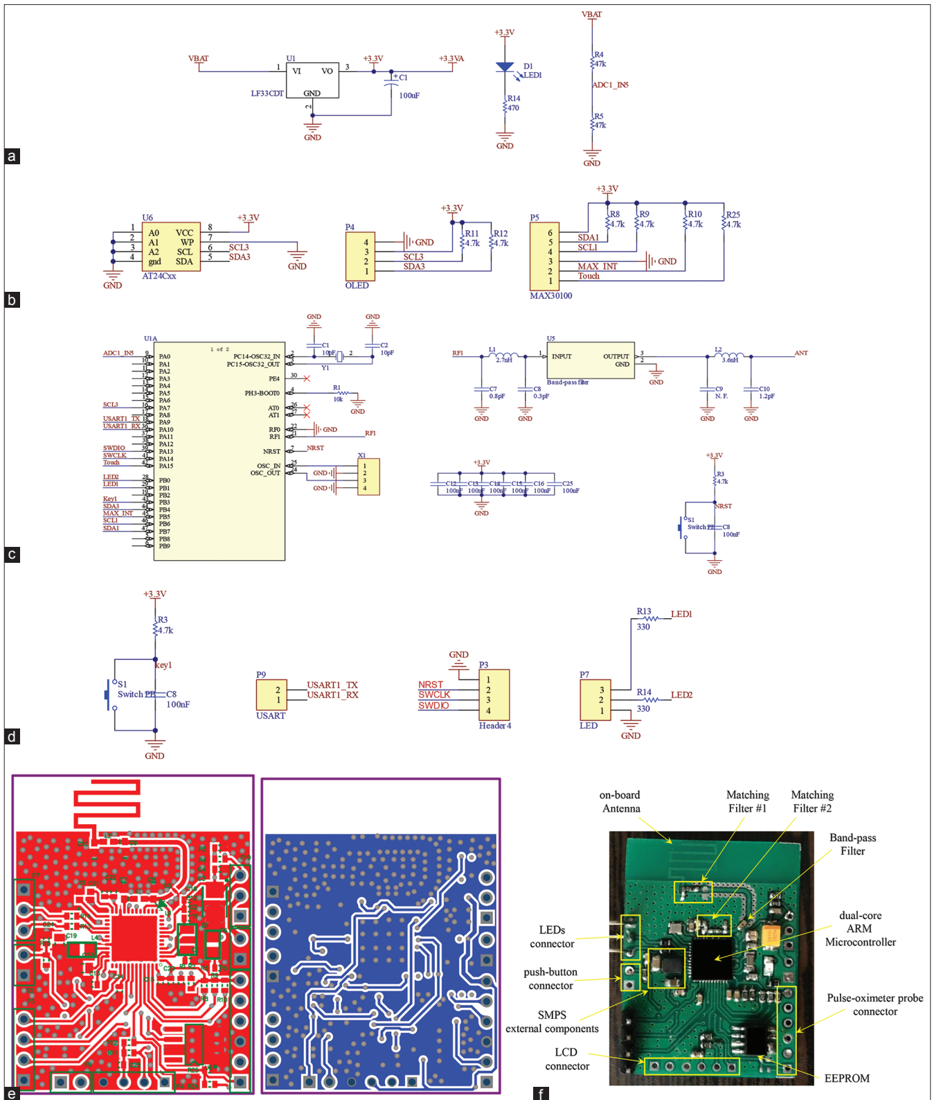
Figure 3: Hardware of the developed wristband: (a) schematic of the voltage regulator, (b) schematics of MAX30100, OLED, and EEPROM, (c) schematic of the microcontroller, (d) schematic of LEDs and a push-button, (e) top and bottom layer of the developed PCB, and (f) implemented wristband's hardware. PCB – Printed circuit board, EEPROM – Electrically erasable programmable read-only memory
