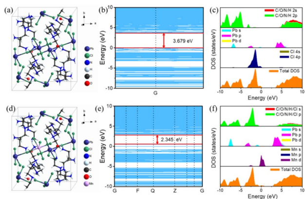
Fig. 5 DFT calculation for pristine and \text{Mn}^{2+} -doped 1D [\text{AEP}]\text{PbCl}_5 \cdot \text{H}_2\text{O} . (a) Unit cell structure, (b) the calculated band structures, and (c) the total and partial density of states for 1D [\text{AEP}]\text{PbCl}_5 \cdot \text{H}_2\text{O} . (d) Unit cell structure, (e) the calculated band structures, and (f) the total and partial density of states for \text{Mn}^{2+} -doped 1D [\text{AEP}]\text{PbCl}_5 \cdot \text{H}_2\text{O} .
