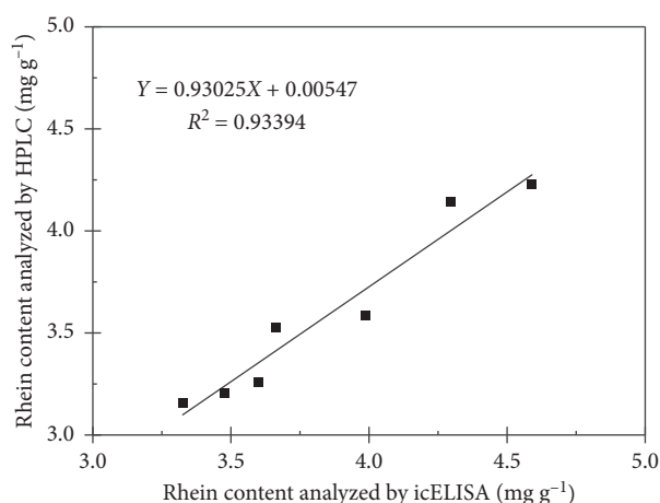
FIGURE 2: Correlation between rhein content of Rheum officinale samples determined by icELISA and by HPLC.
