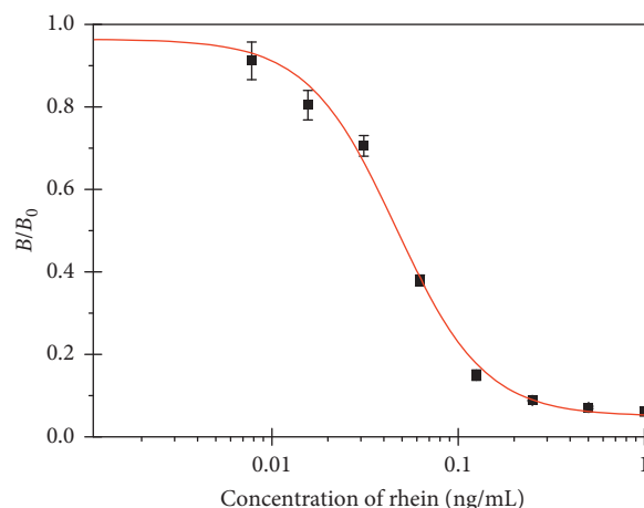
FIGURE 1: Standard inhibition curve of rhein by icELISA, obtained under optimized conditions. B_0 and B were absorbance in the absence and presence of competitors, respectively. Each value represents the mean of three replicates.
