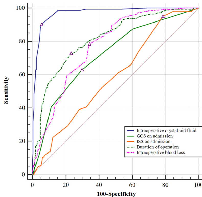
Figure 1 The AUC values for predicting the incidence of postoperative coagulopathy were 0.719 for GCS on admission, 0.589 for ISS on admission, 0.815 for duration of surgery, 0.972 for intraoperative crystalloid fluid volume, and 0.774 for intraoperative blood loss. Δ The cut-off value corresponding to Youden index.
