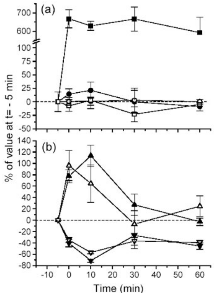
Fig. 4: (a) Time course of total cellular \text{Na}^+ - \text{K}^+ levels in C. raciborskii strain AWT205 cultures exposed to 10 mM NaCl ( \text{Na}^+ = ■, \text{K}^+ = □) in comparison with untreated control samples ( \text{Na}^+ = ●, \text{K}^+ = ○). (b) Effects of STX at 1 \mu\text{M} ( \text{Na}^+ = ▼, \text{K}^+ = ▽) and VTD at 100 \mu\text{M} ( \text{Na}^+ = ▲, \text{K}^+ = △) on total cellular \text{Na}^+ - \text{K}^+ concentrations in C. raciborskii AWT205. Values are expressed as average percentile variation over the sample at -5 min \pm Standard Error.
