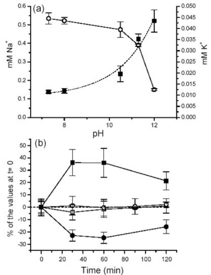
Fig. 2: (a) Total cellular \text{Na}^+ (■) and \text{K}^+ (○) concentrations measured by flame photometry (mM \pm Standard Error in the final cells suspension) in C. raciborskii strain T3 cell suspensions adjusted to different pH and analysed after 2 h. (b) Time course of total cellular \text{Na}^+ - \text{K}^+ levels in C. raciborskii T3 cultures exposed to 10 mM NaCl for 2 h ( \text{Na}^+ = ■, \text{K}^+ = ●), in comparison with untreated samples ( \text{Na}^+ = □, \text{K}^+ = ○); values are expressed as average percentile variation over the sample at 0 min \pm Standard Error.
