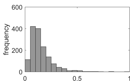
Figure 12. The distribution of reduction factor \alpha .
