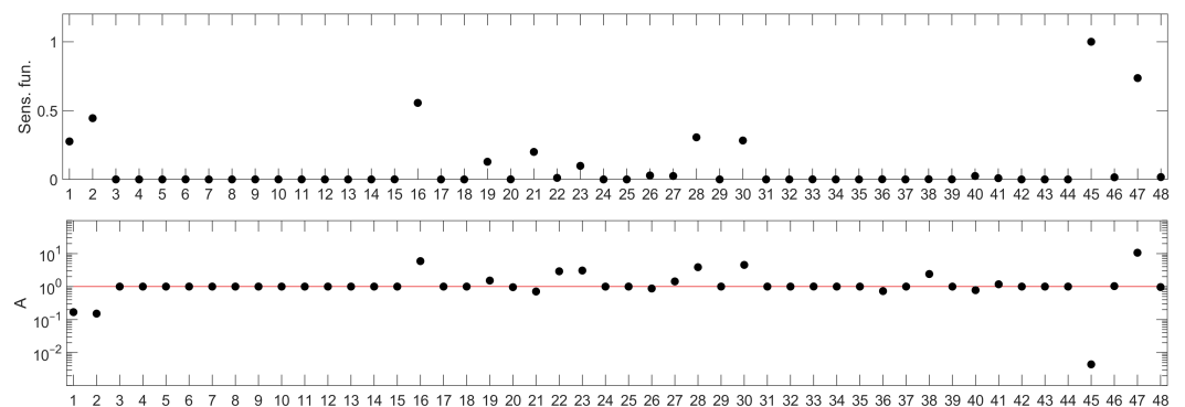
Figure 8. Parameter rankings for IFN- \beta -induced JAK/STAT signaling pathway model: based on sensitivity functions ( top panel ) and based on the method proposed in this paper ( bottom panel ). The horizontal (X) axis represents consecutive model parameters, whose names have been replaced by numbers for better readability. The parameter annotation associated with these numbers is given in Table 2. The red line in the lower panel corresponds to the A index value representing no influence of parameter changes on the model response. Points located above this line represent parameters whose change (as described in the algorithm details) amplify the model response, while those below represent the parameters whose change lead to the suppression of the model response.
