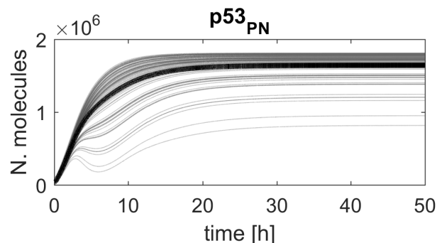
Figure 4. Simulated p53 protein responses in the model with parameter t_0 altered by the reduction factor \alpha . The figure shows 100 randomly selected p53 protein responses (gray lines) and average p53 protein responses (black line) calculated from 1000 simulations.
