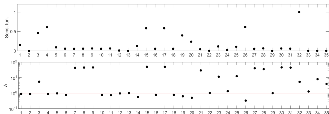
Figure 2. Parameter rankings for the p53 model: based on sensitivity functions ( upper panel ) and based on the method proposed in this paper ( lower panel ). The horizontal (X) axis represents the consecutive model parameters, whose names have been replaced by numbers for better readability. The parameter annotation associated with these numbers is given in Table 1. The red line in the lower panel corresponds to the A index value representing no influence of parameter change on the model response. Points located above this line represent parameters whose change (as described in the algorithm details) amplify the model response, while those below represent the parameters whose change lead to suppression of the model response.
